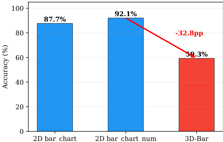
2D vs 3D Bar Chart Accuracy
